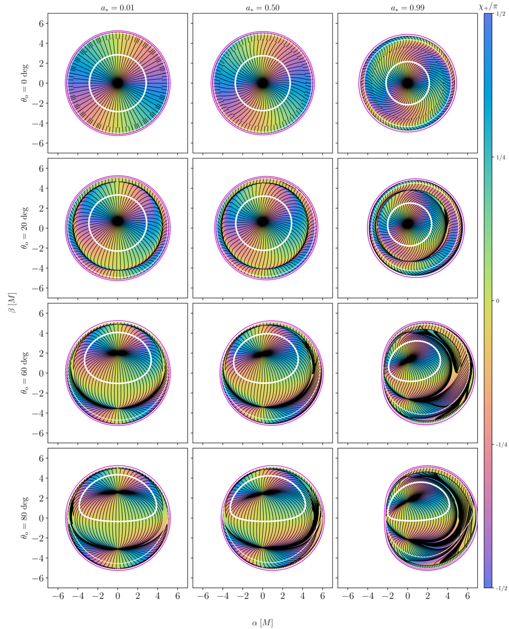
Figure 2. from Andrew Chael et al 2026 Astrophys. J. Lett. 1009 doi:10.3847/2041-8213/ae9ebf https://dx.doi.org/10.3847/2041-8213/ae9ebf © 2026. The Author(s). Published by the American Astronomical Society.
