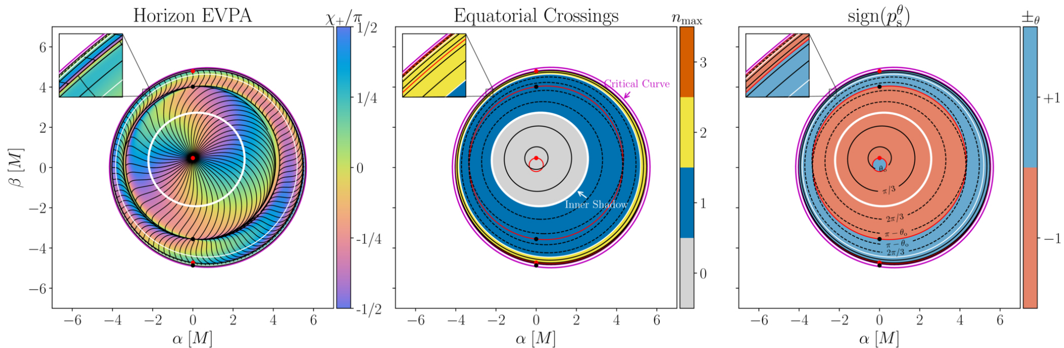
Figure 1. from Andrew Chael et al 2026 Astrophys. J. Lett. 1009 doi:10.3847/2041-8213/ae9ebf https://dx.doi.org/10.3847/2041-8213/ae9ebf © 2026. The Author(s). Published by the American Astronomical Society.
