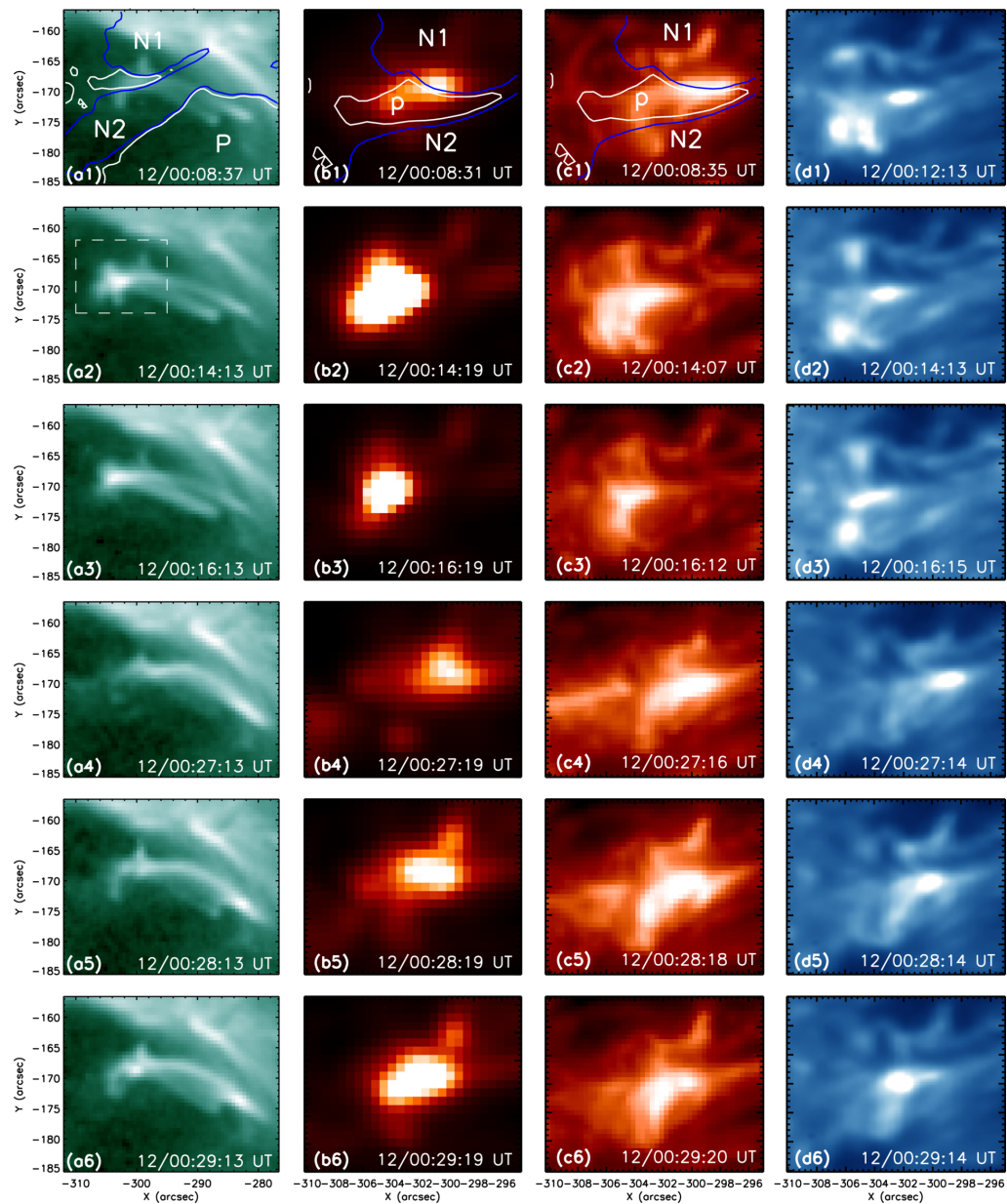
Figure 4. from Bo Yang et al 2026 Astrophys. J. Lett. 1008 doi:10.3847/2041-8213/ae9ebe https://dx.doi.org/10.3847/2041-8213/ae9ebe © 2026. The Author(s). Published by the American Astronomical Society.
