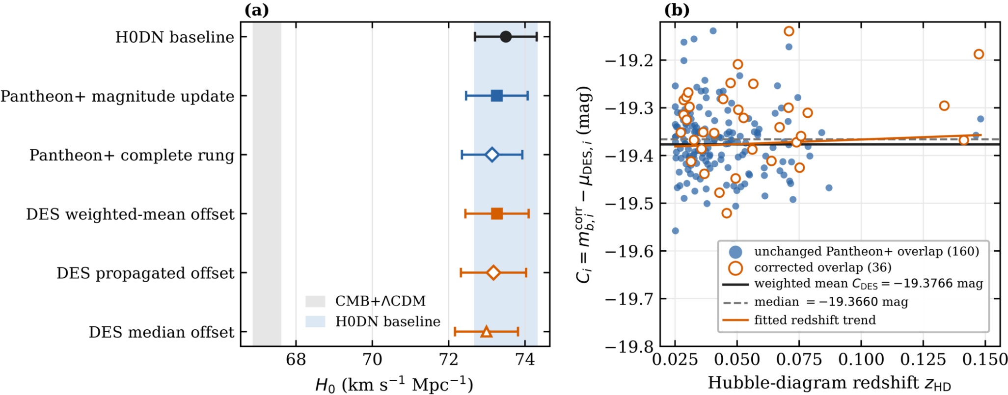
Figure 1. from Shouvik Roy Choudhury 2026 Astrophys. J. Lett. 1008 doi:10.3847/2041-8213/ae9d80 https://dx.doi.org/10.3847/2041-8213/ae9d80 © 2026. The Author(s). Published by the American Astronomical Society.
