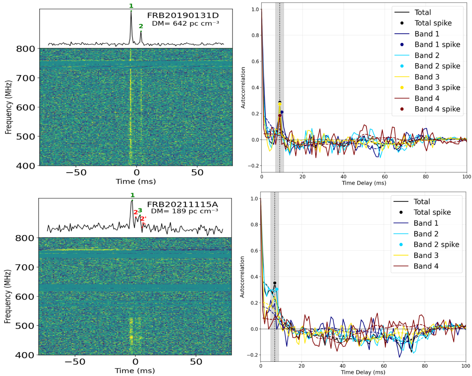
Figure 4. from Huan Zhou et al 2026 Astrophys. J. Lett. 1008 doi:10.3847/2041-8213/ae9d75 https://dx.doi.org/10.3847/2041-8213/ae9d75 © 2026. The Author(s). Published by the American Astronomical Society.
