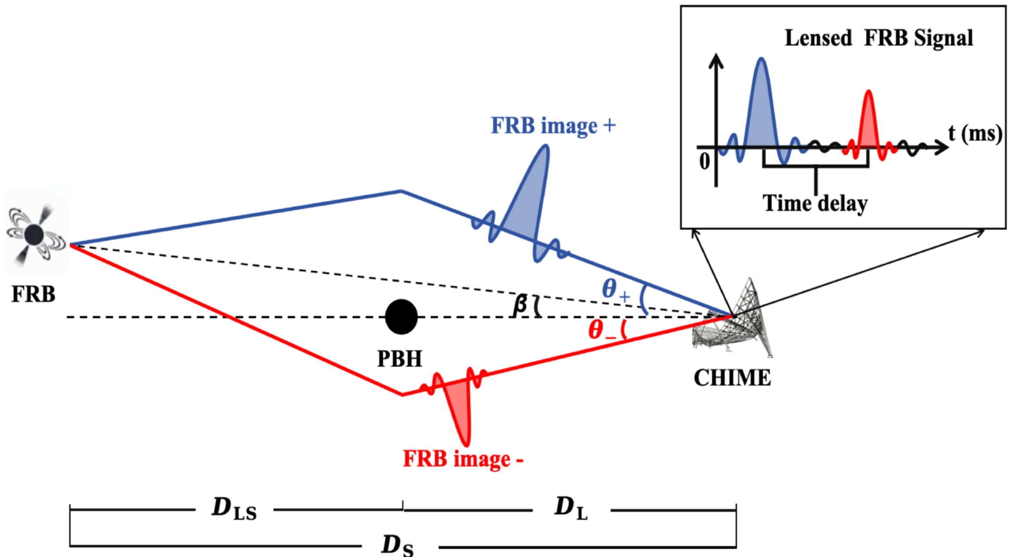
Figure 2. from Huan Zhou et al 2026 Astrophys. J. Lett. 1008 doi:10.3847/2041-8213/ae9d75 https://dx.doi.org/10.3847/2041-8213/ae9d75 © 2026. The Author(s). Published by the American Astronomical Society.
