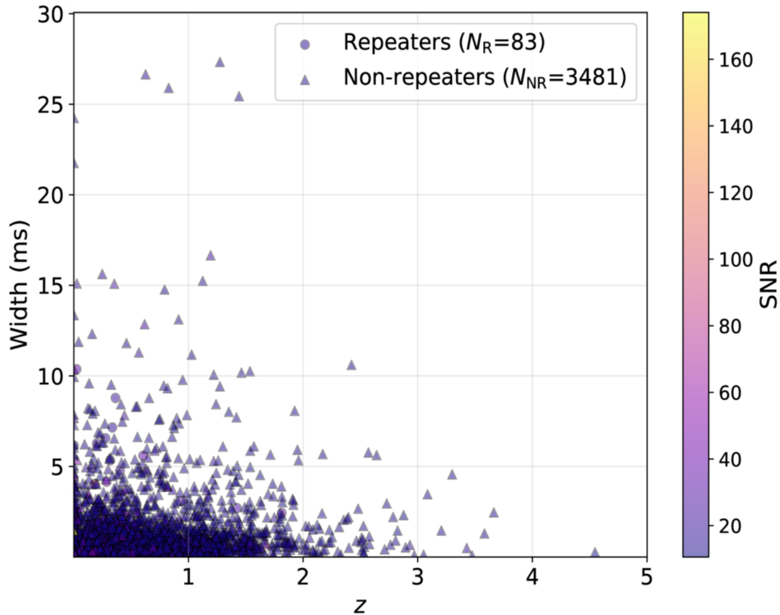
Figure 1. from Huan Zhou et al 2026 Astrophys. J. Lett. 1008 doi:10.3847/2041-8213/ae9d75 https://dx.doi.org/10.3847/2041-8213/ae9d75 © 2026. The Author(s). Published by the American Astronomical Society.
