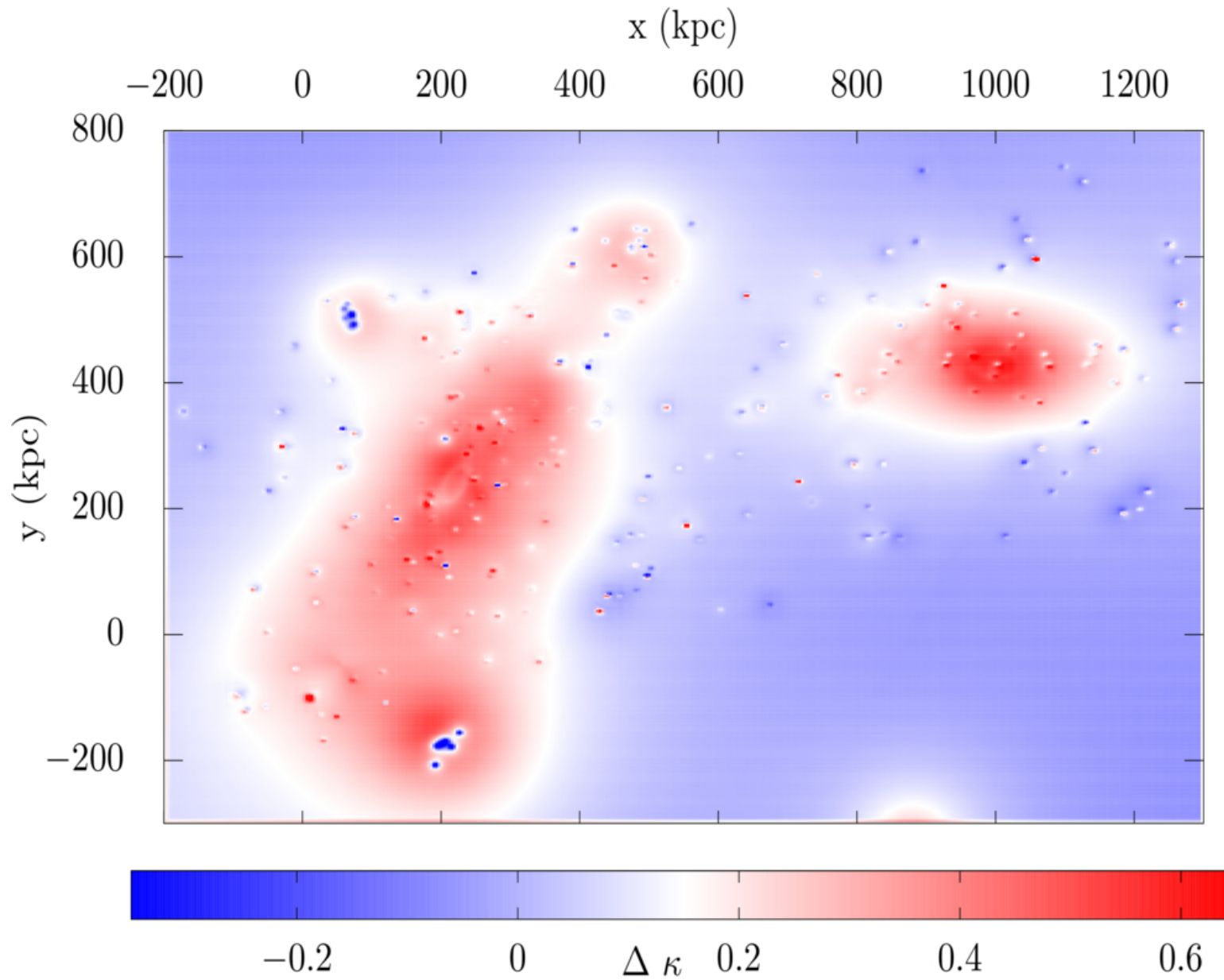
Figure 2. from X. Hernandez 2026 Astrophys. J. Lett. 1008 doi:10.3847/2041-8213/ae9d4c https://dx.doi.org/10.3847/2041-8213/ae9d4c © 2026. The Author(s). Published by the American Astronomical Society.
