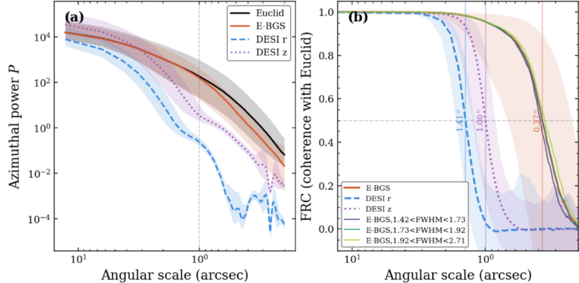
Figure 4. from Renhao Ye et al 2026 Astrophys. J. Lett. 1009 doi:10.3847/2041-8213/ae9cbf https://dx.doi.org/10.3847/2041-8213/ae9cbf © 2026. The Author(s). Published by the American Astronomical Society.
