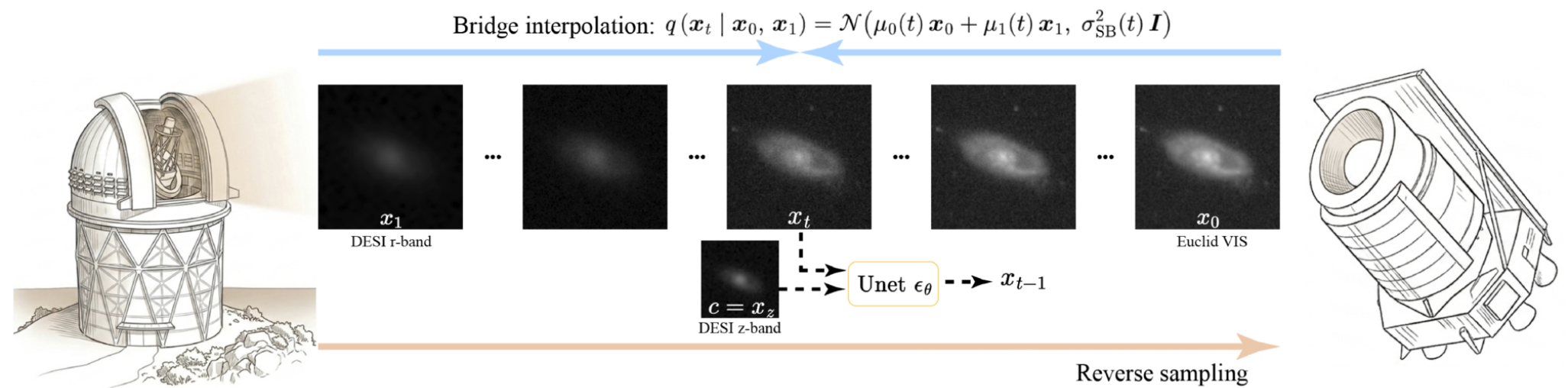
Figure 2. from Renhao Ye et al 2026 Astrophys. J. Lett. 1009 doi:10.3847/2041-8213/ae9cbf https://dx.doi.org/10.3847/2041-8213/ae9cbf © 2026. The Author(s). Published by the American Astronomical Society.
