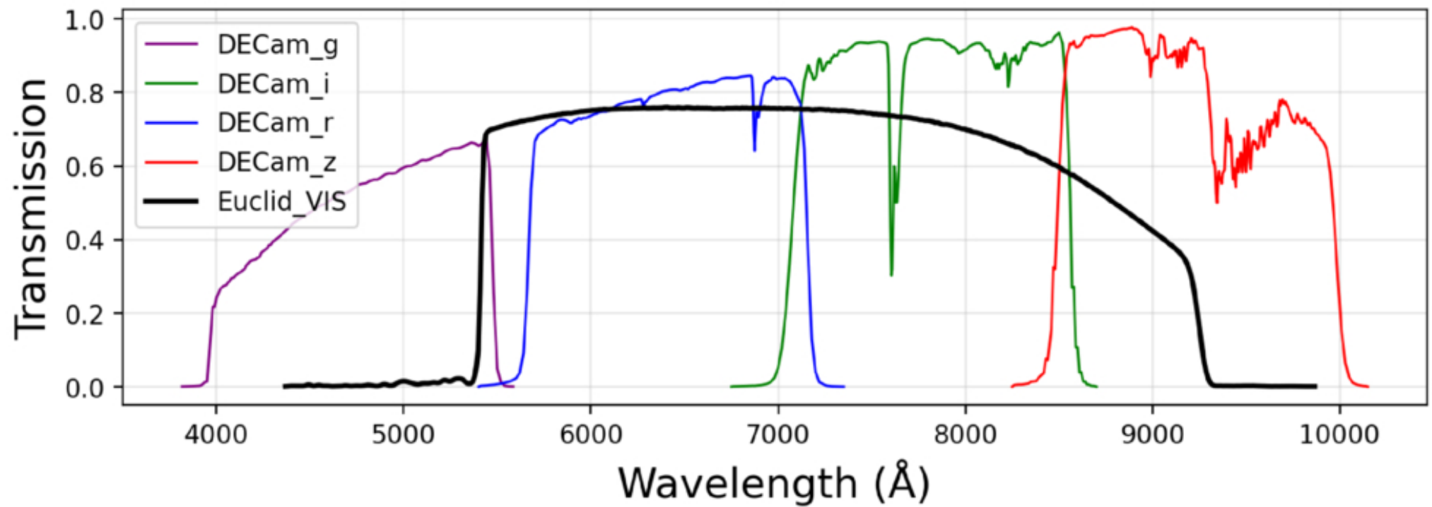
Figure 1. from Renhao Ye et al 2026 Astrophys. J. Lett. 1009 doi:10.3847/2041-8213/ae9cbf https://dx.doi.org/10.3847/2041-8213/ae9cbf © 2026. The Author(s). Published by the American Astronomical Society.
