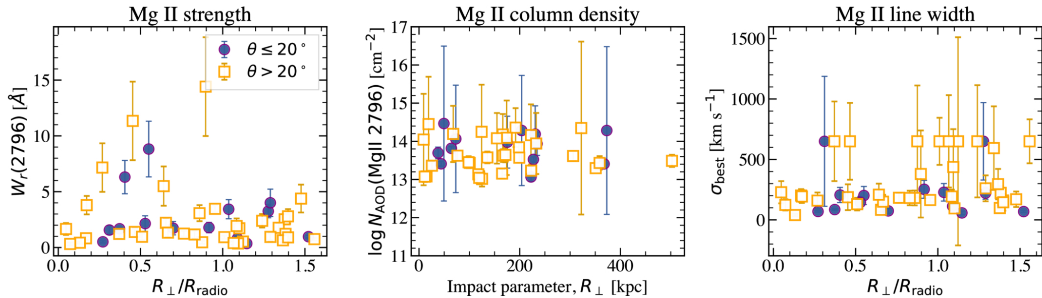
Figure 4. from Namrata Roy et al 2026 Astrophys. J. Lett. 1009 doi:10.3847/2041-8213/ae9cbd https://dx.doi.org/10.3847/2041-8213/ae9cbd © 2026. The Author(s). Published by the American Astronomical Society.
