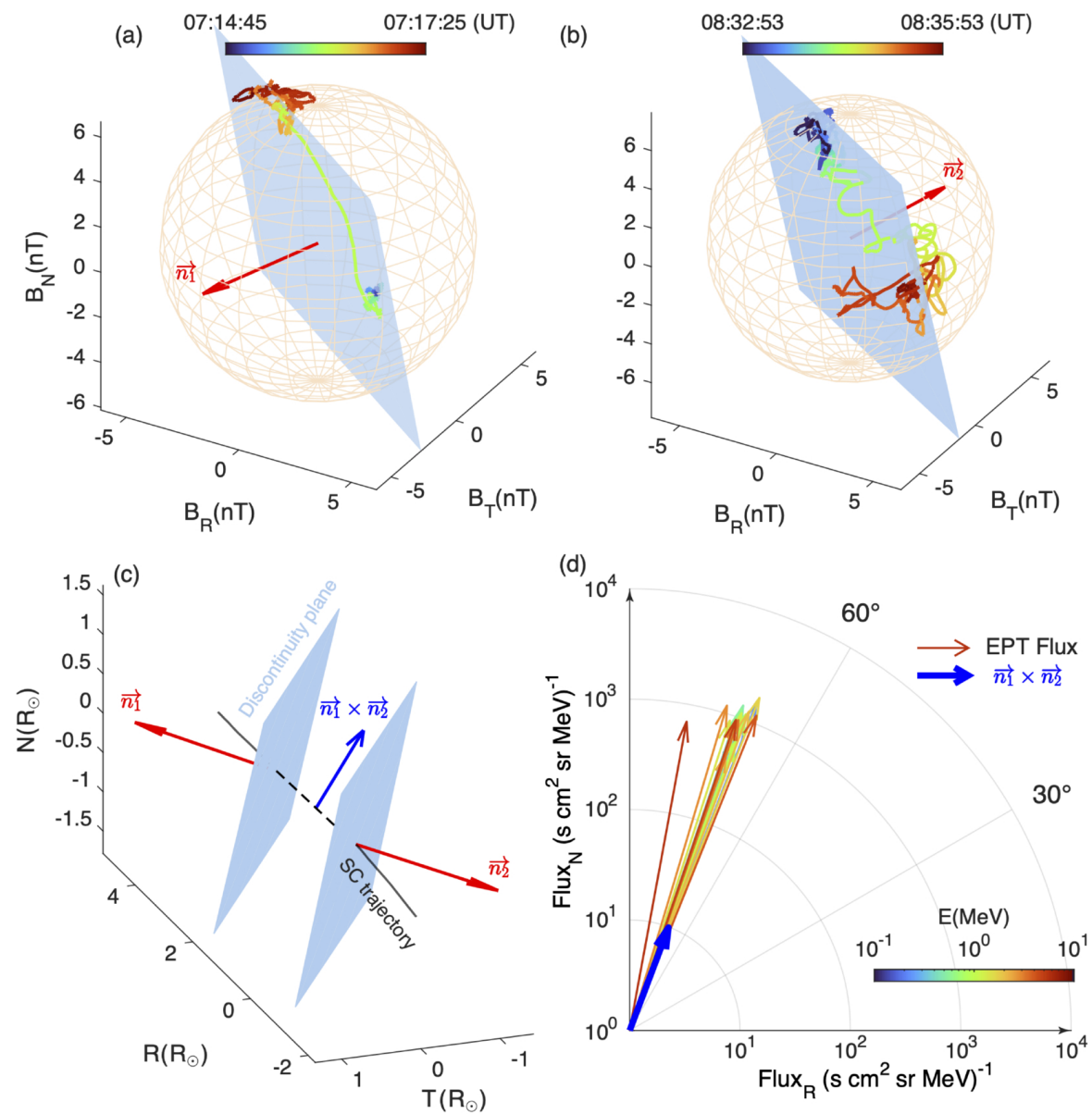
Figure 4. from Xiaohang Chen et al 2026 Astrophys. J. Lett. 1008 doi:10.3847/2041-8213/ae9cba https://dx.doi.org/10.3847/2041-8213/ae9cba © 2026. The Author(s). Published by the American Astronomical Society.
