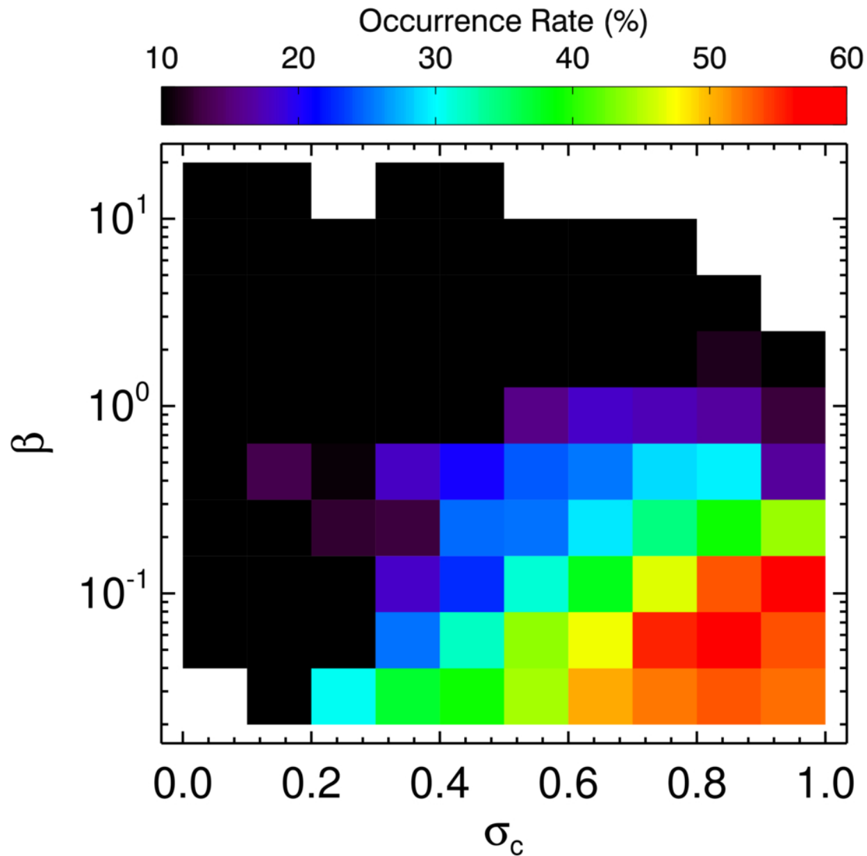
Figure 3. from G. Q. Zhao et al 2026 Astrophys. J. Lett. 1008 doi:10.3847/2041-8213/ae9cb4 https://dx.doi.org/10.3847/2041-8213/ae9cb4 © 2026. The Author(s). Published by the American Astronomical Society.
