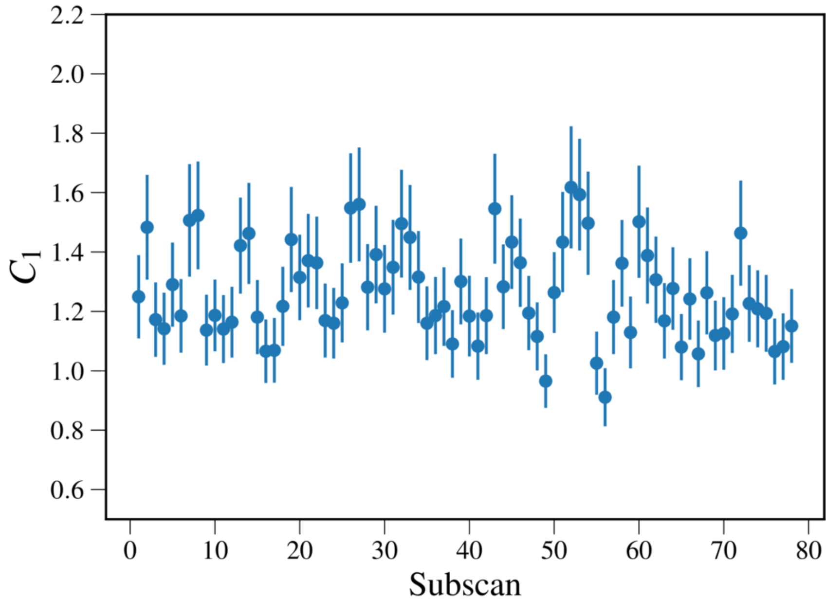
Figure 2. from Jacob E. Turner 2026 Astrophys. J. Lett. 1008 doi:10.3847/2041-8213/ae9c3e https://dx.doi.org/10.3847/2041-8213/ae9c3e © 2026. The Author(s). Published by the American Astronomical Society.
