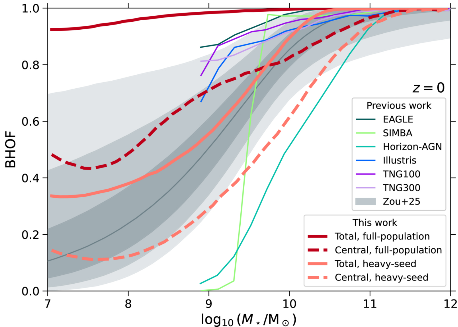
Figure 5. from Emma Jane Weller et al 2026 Astrophys. J. Lett. 1008 doi:10.3847/2041-8213/ae9c38 https://dx.doi.org/10.3847/2041-8213/ae9c38 © 2026. The Author(s). Published by the American Astronomical Society.
