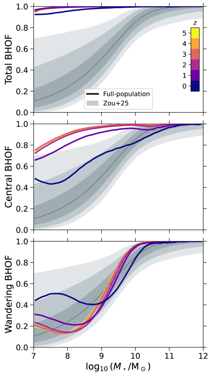
Figure 2. from Emma Jane Weller et al 2026 Astrophys. J. Lett. 1008 doi:10.3847/2041-8213/ae9c38 https://dx.doi.org/10.3847/2041-8213/ae9c38 © 2026. The Author(s). Published by the American Astronomical Society.
