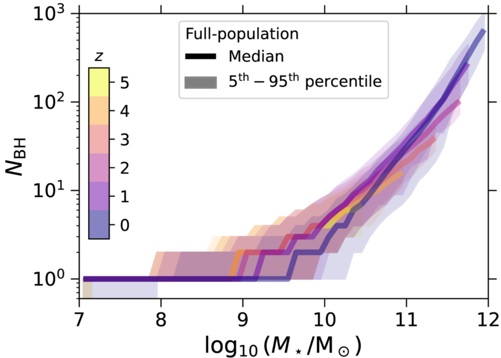
Figure 1. from Emma Jane Weller et al 2026 Astrophys. J. Lett. 1008 doi:10.3847/2041-8213/ae9c38 https://dx.doi.org/10.3847/2041-8213/ae9c38 © 2026. The Author(s). Published by the American Astronomical Society.
