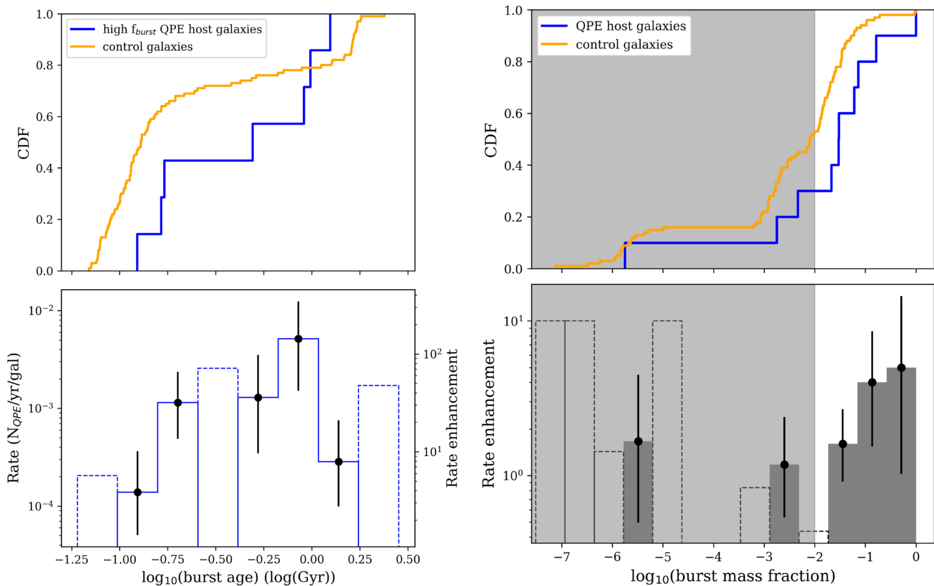
Figure 2. from Margaret Shepherd et al 2026 Astrophys. J. Lett. 1008 doi:10.3847/2041-8213/ae9c30 https://dx.doi.org/10.3847/2041-8213/ae9c30 © 2026. The Author(s). Published by the American Astronomical Society.
