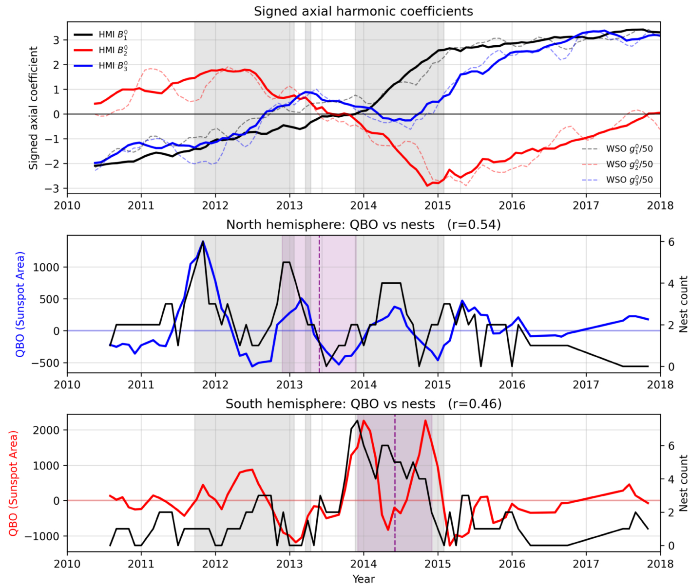
Figure 4. Signed Axial Harmonic Coefficients and Hemispheric QBO–Nest Comparison from A. A. Norton 2026 Astrophys. J. Lett. 1009 doi:10.3847/2041-8213/ae9bac https://dx.doi.org/10.3847/2041-8213/ae9bac © 2026. The Author(s). Published by the American Astronomical Society.
