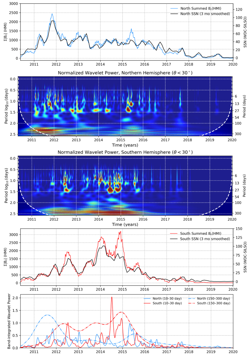
Figure 1. from A. A. Norton 2026 Astrophys. J. Lett. 1009 doi:10.3847/2041-8213/ae9bac https://dx.doi.org/10.3847/2041-8213/ae9bac © 2026. The Author(s). Published by the American Astronomical Society.
