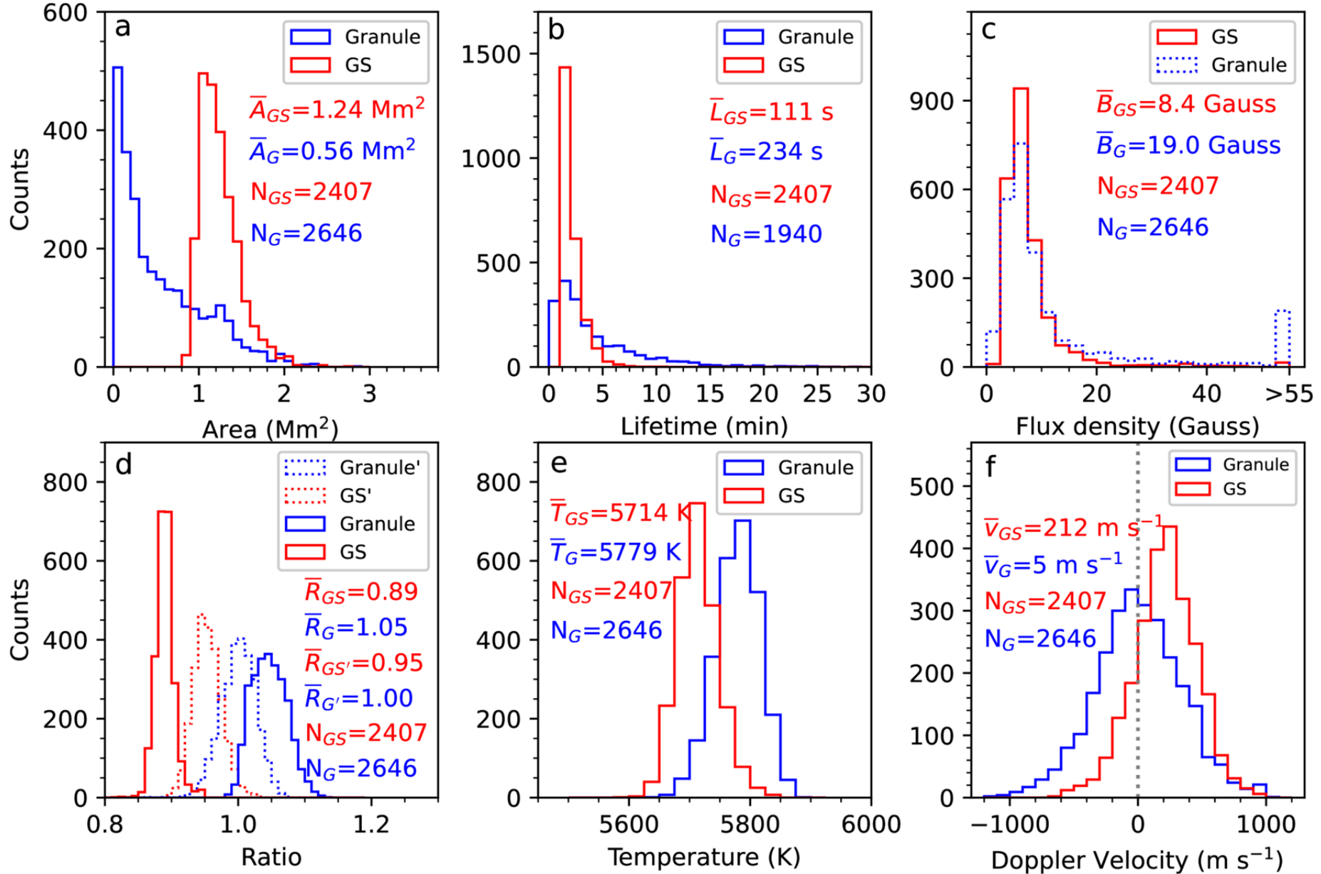
Figure 6. from Shaoxuan Tong et al 2026 Astrophys. J. Lett. 1008 doi:10.3847/2041-8213/ae9ba9 https://dx.doi.org/10.3847/2041-8213/ae9ba9 © 2026. The Author(s). Published by the American Astronomical Society.
