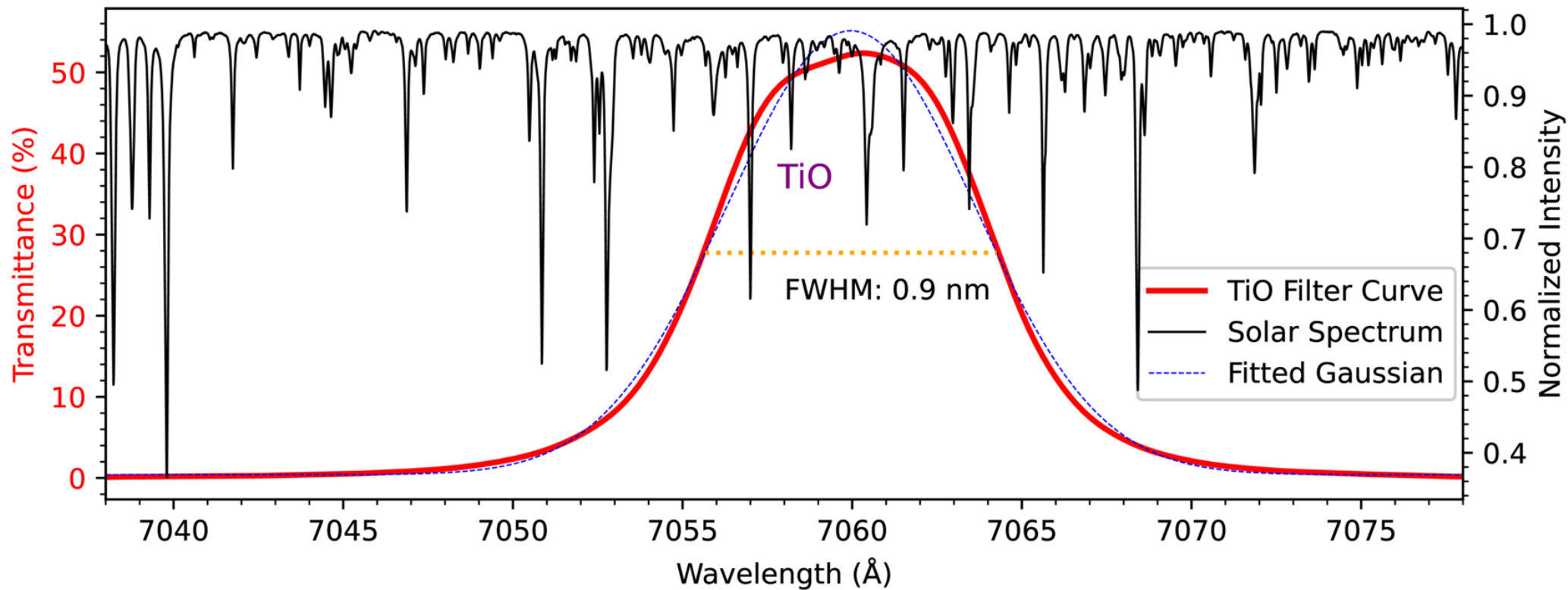
Figure 1. from Shaoxuan Tong et al 2026 Astrophys. J. Lett. 1008 doi:10.3847/2041-8213/ae9ba9 https://dx.doi.org/10.3847/2041-8213/ae9ba9 © 2026. The Author(s). Published by the American Astronomical Society.
