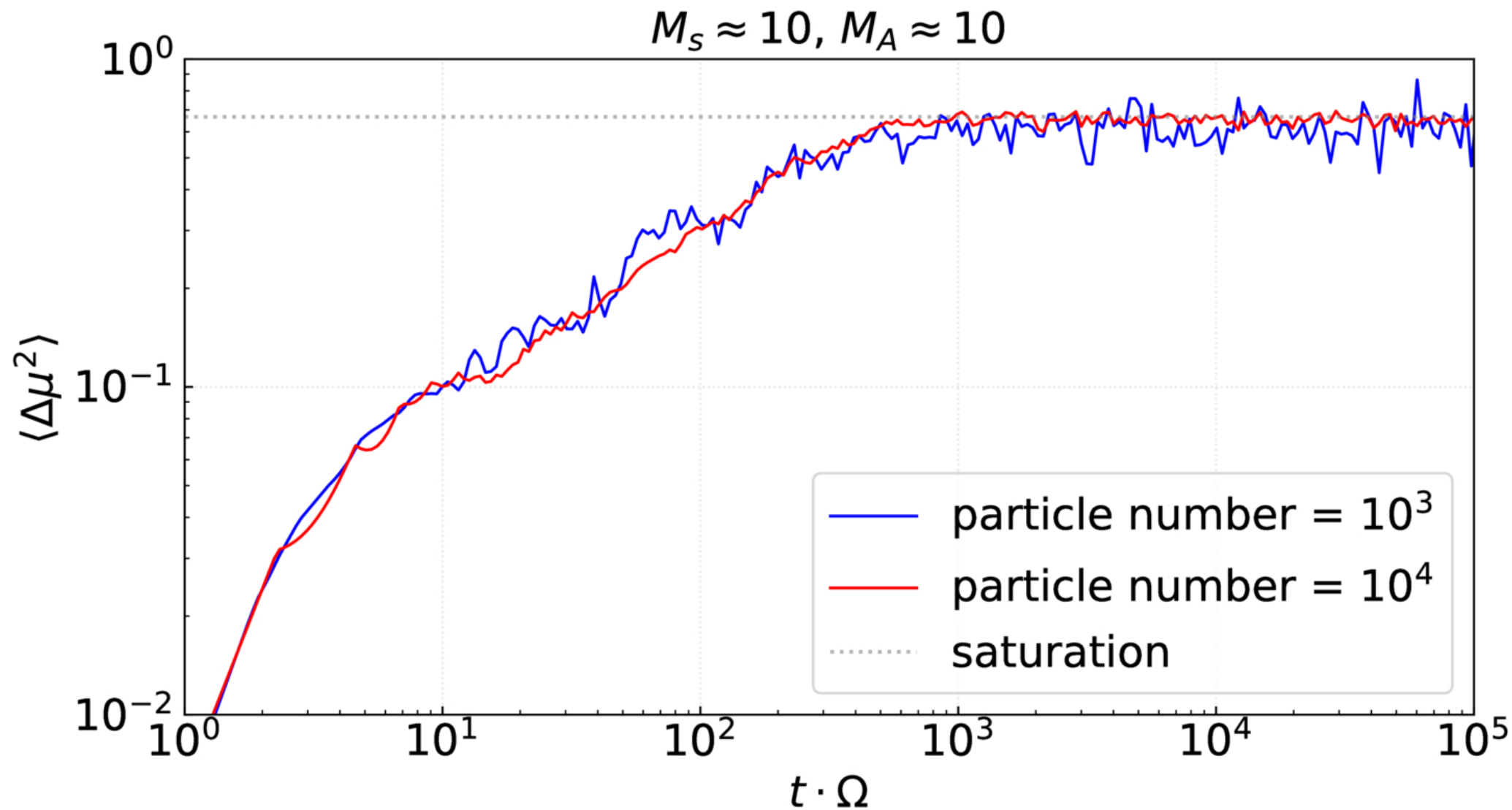
Figure A1. from Yue Hu 2026 Astrophys. J. Lett. 1008 doi:10.3847/2041-8213/ae9ba5 https://dx.doi.org/10.3847/2041-8213/ae9ba5 © 2026. The Author(s). Published by the American Astronomical Society.
