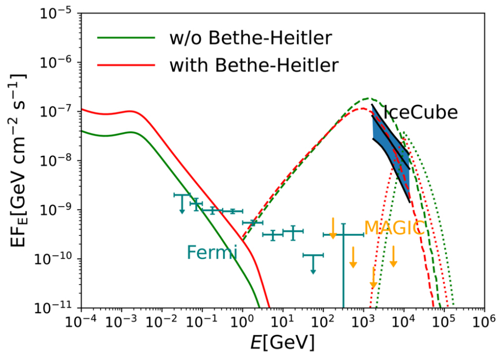
(a) pp + p\gamma
