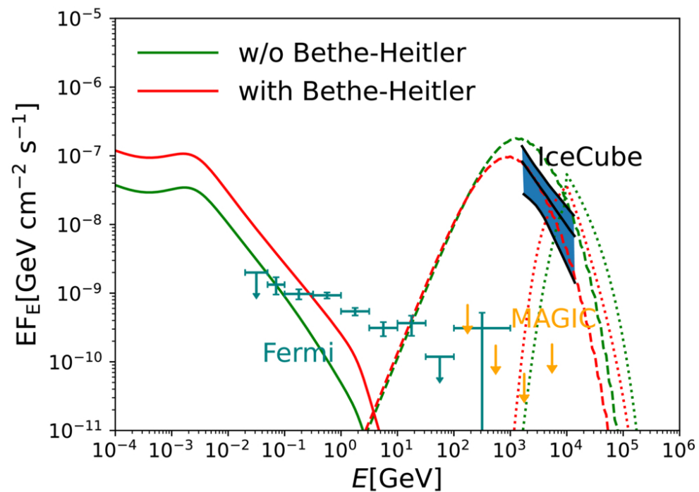
(b) p\gamma only
