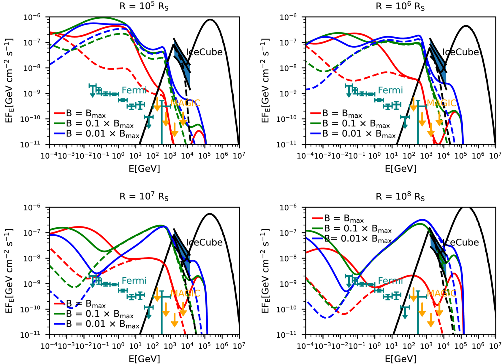
Figure 5. from Abhishek Das et al 2026 Astrophys. J. Lett. 1009 doi:10.3847/2041-8213/ae9ba3 https://dx.doi.org/10.3847/2041-8213/ae9ba3 © 2026. The Author(s). Published by the American Astronomical Society.
