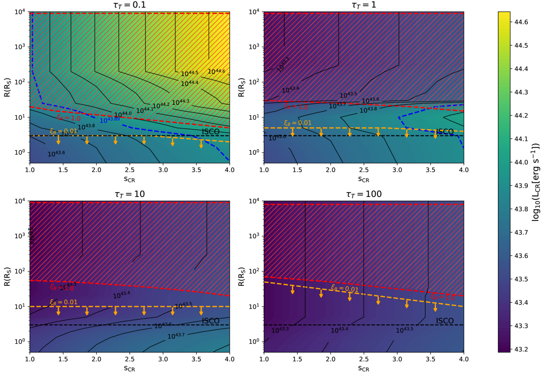
Figure 4. from Abhishek Das et al 2026 Astrophys. J. Lett. 1009 doi:10.3847/2041-8213/ae9ba3 https://dx.doi.org/10.3847/2041-8213/ae9ba3 © 2026. The Author(s). Published by the American Astronomical Society.
