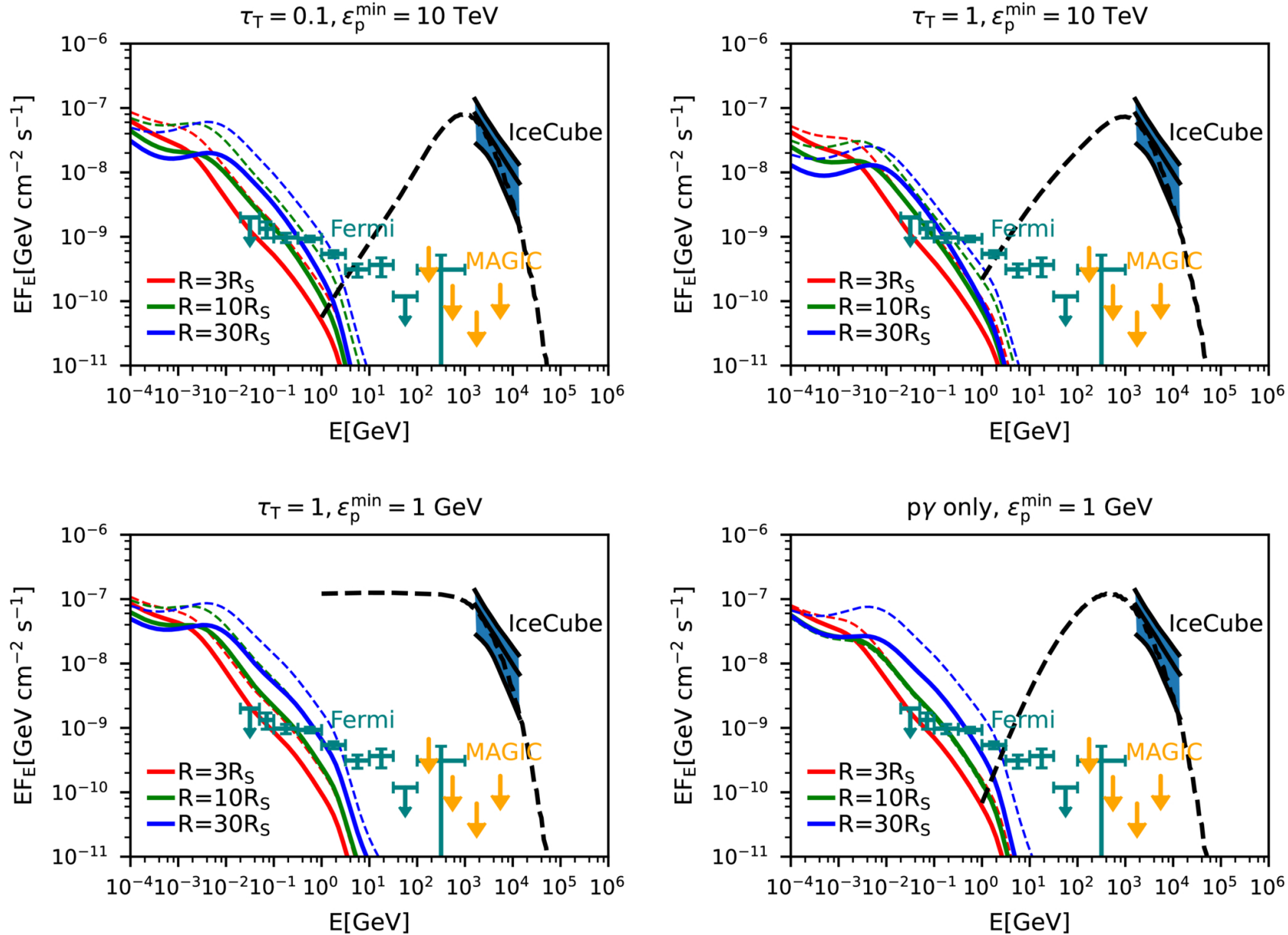
Figure 2. from Abhishek Das et al 2026 Astrophys. J. Lett. 1009 doi:10.3847/2041-8213/ae9ba3 https://dx.doi.org/10.3847/2041-8213/ae9ba3 © 2026. The Author(s). Published by the American Astronomical Society.
