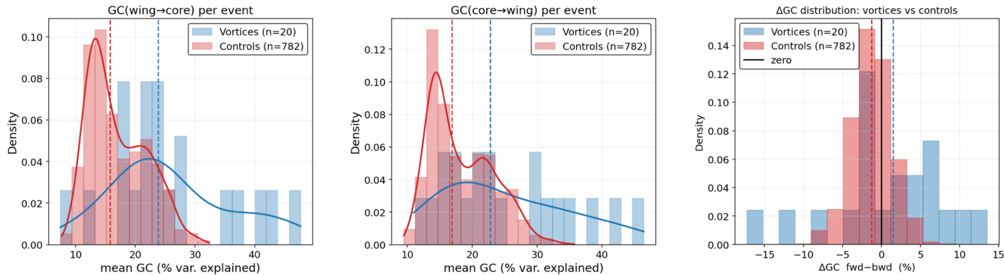
Figure 5. from Suzana S. A. Silva et al 2026 Astrophys. J. Lett. 1008 doi:10.3847/2041-8213/ae9b0b https://dx.doi.org/10.3847/2041-8213/ae9b0b © 2026. The Author(s). Published by the American Astronomical Society.
