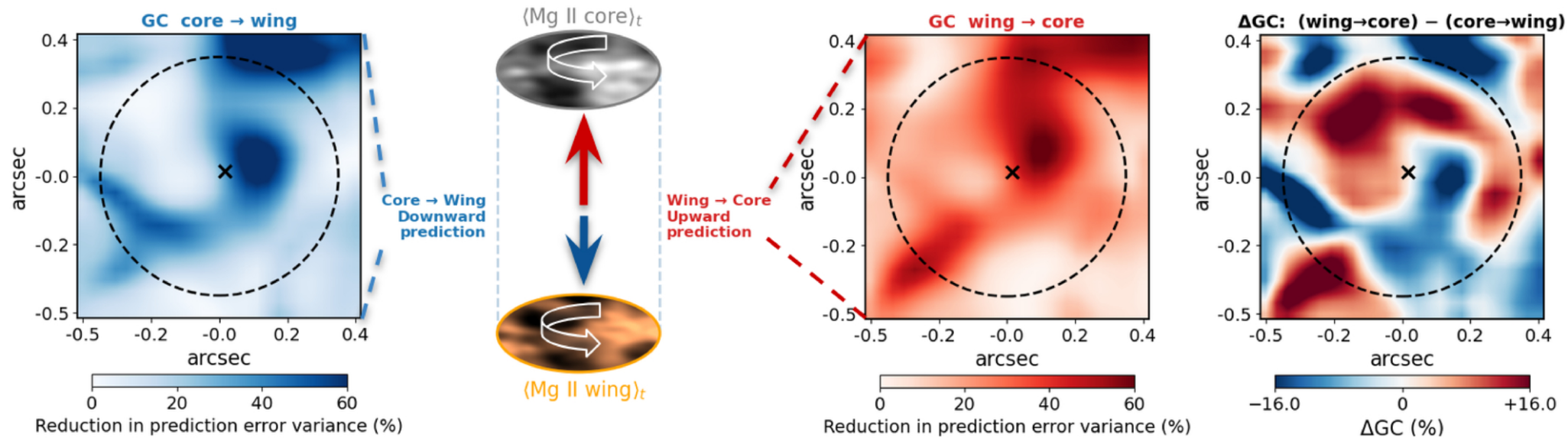
Figure 4. from Suzana S. A. Silva et al 2026 Astrophys. J. Lett. 1008 doi:10.3847/2041-8213/ae9b0b https://dx.doi.org/10.3847/2041-8213/ae9b0b © 2026. The Author(s). Published by the American Astronomical Society.
