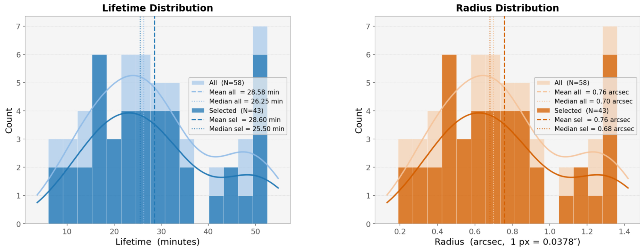
Figure 3. from Suzana S. A. Silva et al 2026 Astrophys. J. Lett. 1008 doi:10.3847/2041-8213/ae9b0b https://dx.doi.org/10.3847/2041-8213/ae9b0b © 2026. The Author(s). Published by the American Astronomical Society.
