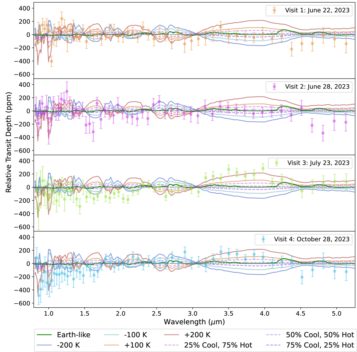
Figure 5. from Ana Glidden et al 2026 Astrophys. J. Lett. 1008 doi:10.3847/2041-8213/ae9b0a https://dx.doi.org/10.3847/2041-8213/ae9b0a © 2026. The Author(s). Published by the American Astronomical Society.
