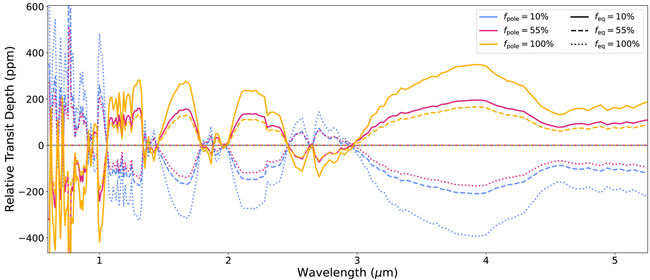
Figure 3. from Ana Glidden et al 2026 Astrophys. J. Lett. 1008 doi:10.3847/2041-8213/ae9b0a https://dx.doi.org/10.3847/2041-8213/ae9b0a © 2026. The Author(s). Published by the American Astronomical Society.
