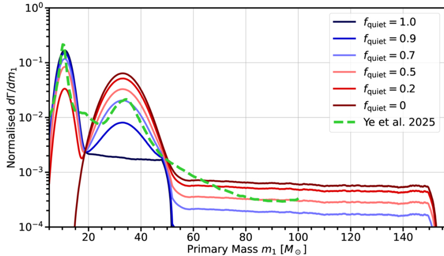
(c) Different accretion fractions
