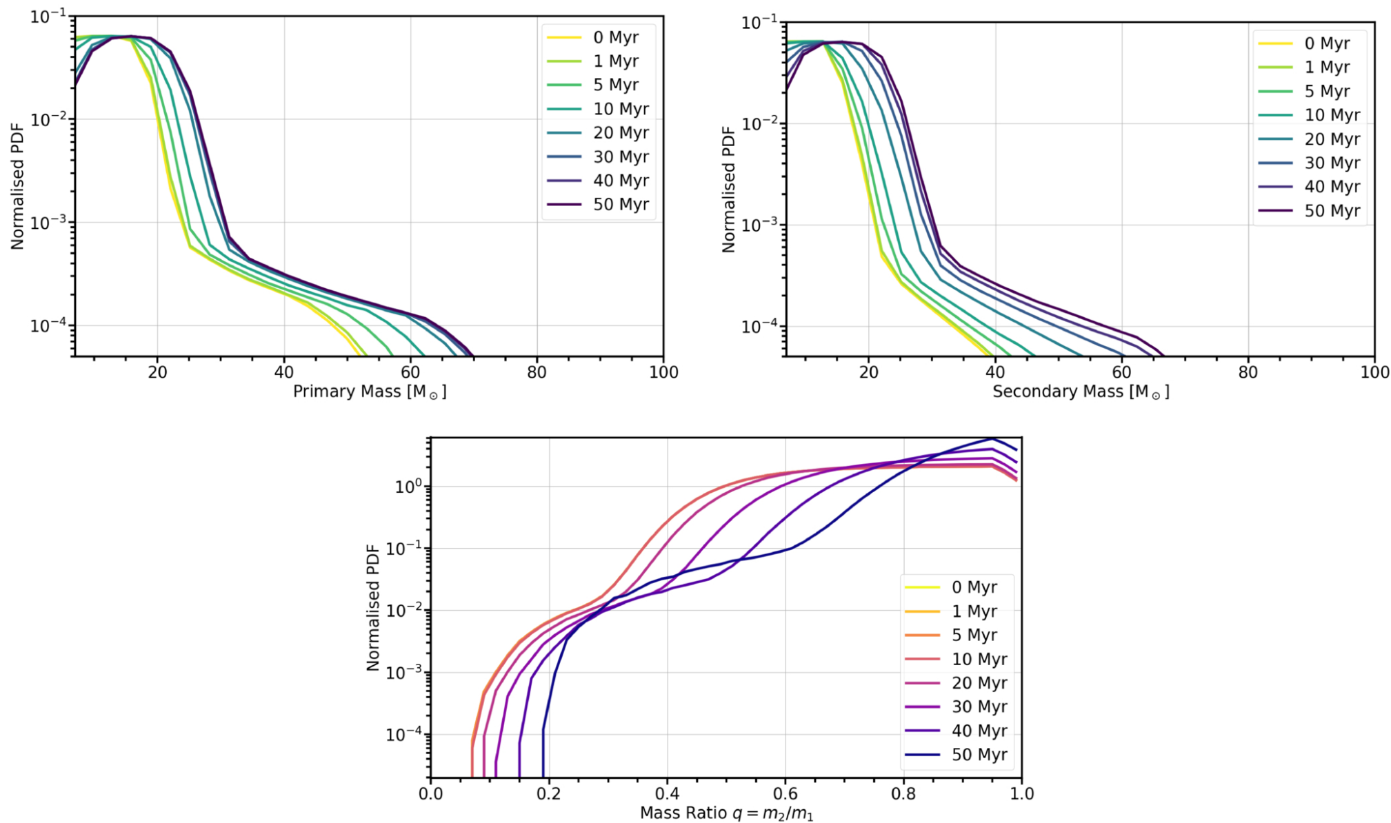
Figure 4. from Mor Rozner et al 2026 Astrophys. J. Lett. 1008 doi:10.3847/2041-8213/ae9b08 https://dx.doi.org/10.3847/2041-8213/ae9b08 © 2026. The Author(s). Published by the American Astronomical Society.
