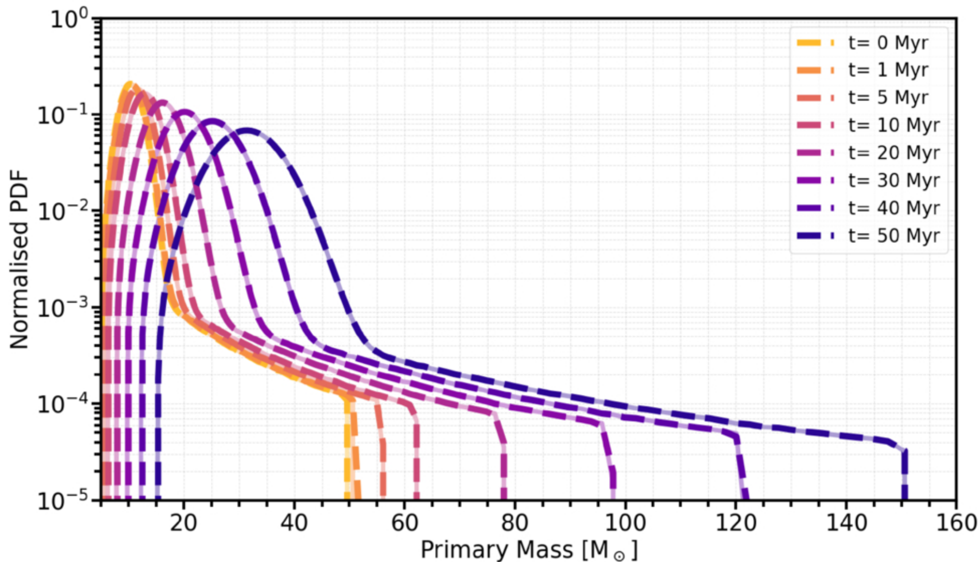
Figure 2. from Mor Rozner et al 2026 Astrophys. J. Lett. 1008 doi:10.3847/2041-8213/ae9b08 https://dx.doi.org/10.3847/2041-8213/ae9b08 © 2026. The Author(s). Published by the American Astronomical Society.
