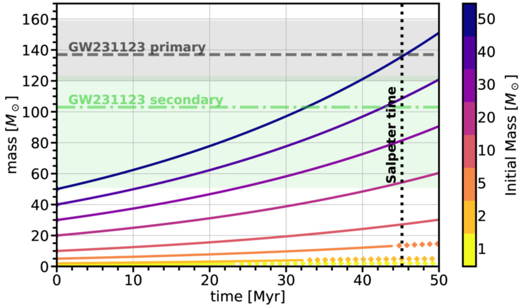
Figure 1. from Mor Rozner et al 2026 Astrophys. J. Lett. 1008 doi:10.3847/2041-8213/ae9b08 https://dx.doi.org/10.3847/2041-8213/ae9b08 © 2026. The Author(s). Published by the American Astronomical Society.
