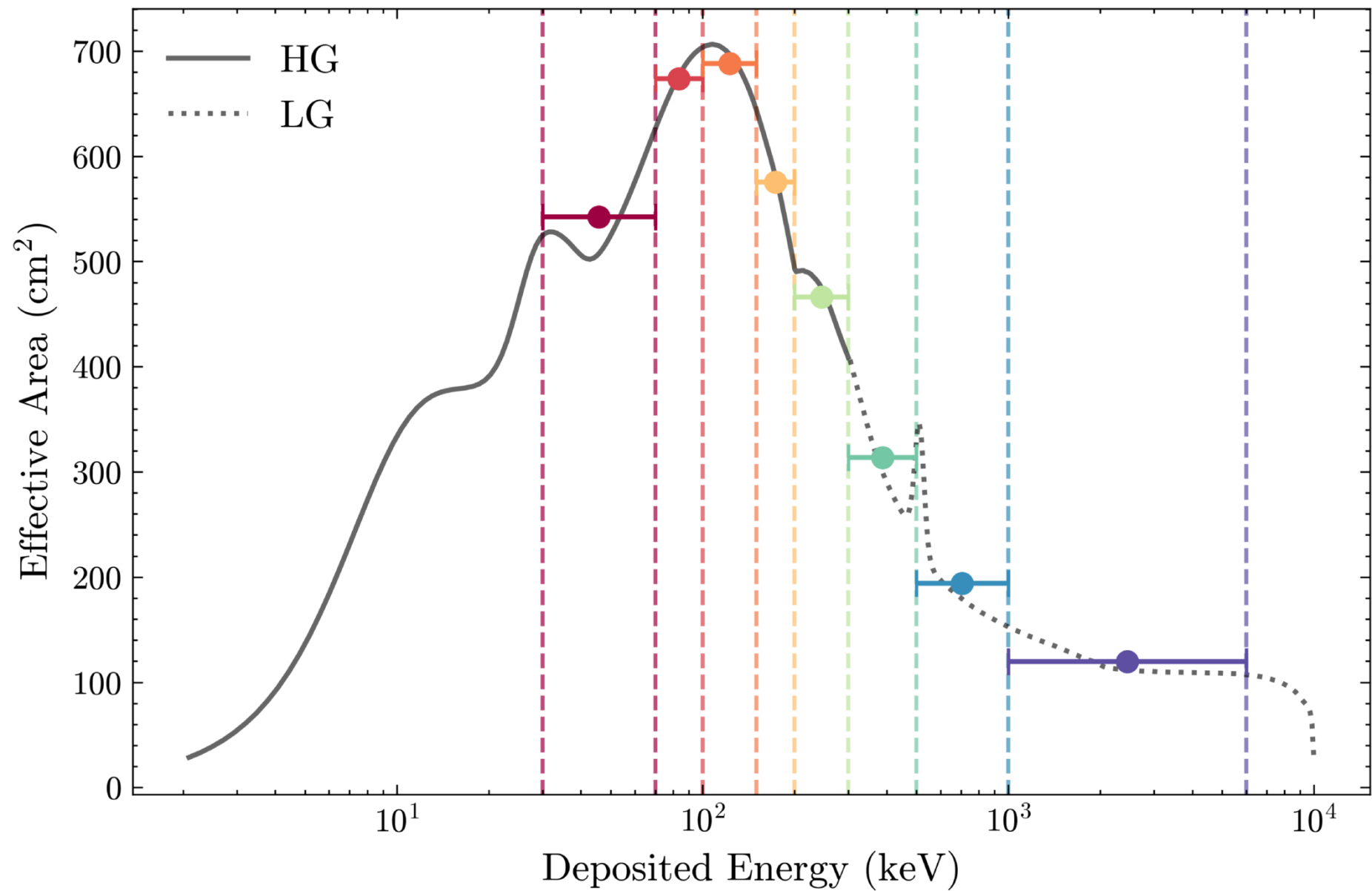
Figure A1. from Wen-Long Zhang et al 2026 Astrophys. J. Lett. 1009 doi:10.3847/2041-8213/ae9b03 https://dx.doi.org/10.3847/2041-8213/ae9b03 © 2026. The Author(s). Published by the American Astronomical Society.
