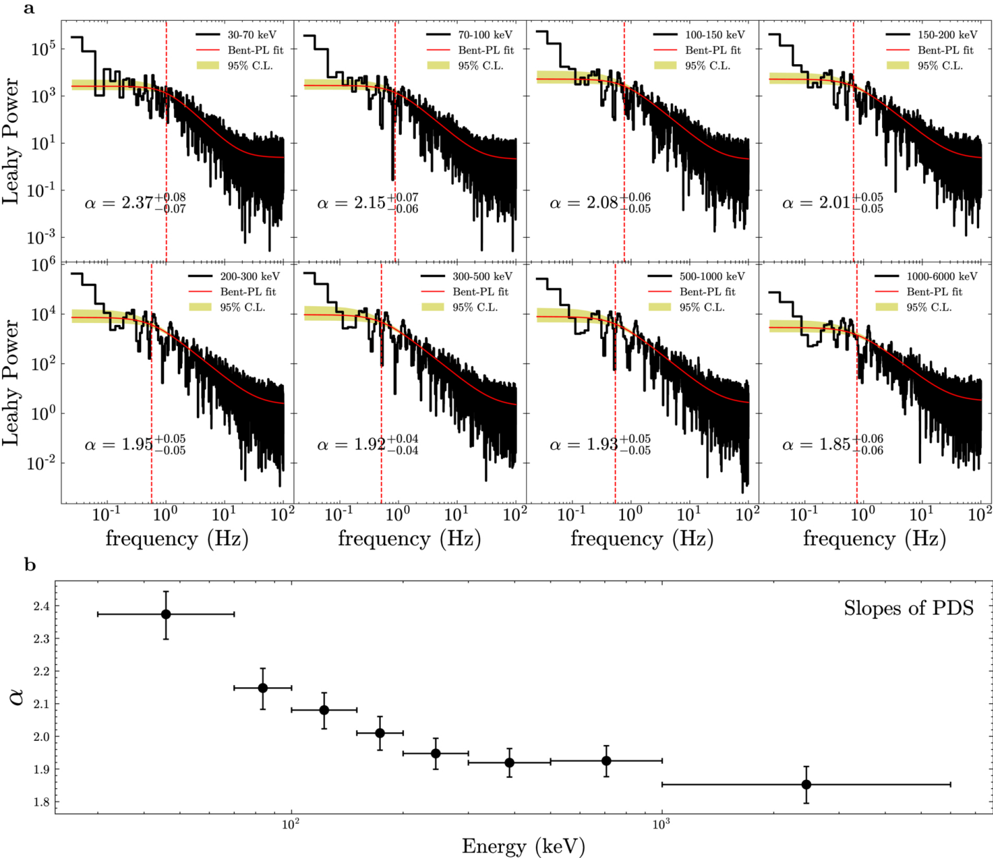
Figure 5. from Wen-Long Zhang et al 2026 Astrophys. J. Lett. 1009 doi:10.3847/2041-8213/ae9b03 https://dx.doi.org/10.3847/2041-8213/ae9b03 © 2026. The Author(s). Published by the American Astronomical Society.
