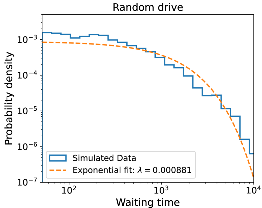
Figure A5. from Wen-Long Zhang et al 2026 Astrophys. J. Lett. 1009 doi:10.3847/2041-8213/ae9b03 https://dx.doi.org/10.3847/2041-8213/ae9b03 © 2026. The Author(s). Published by the American Astronomical Society.
