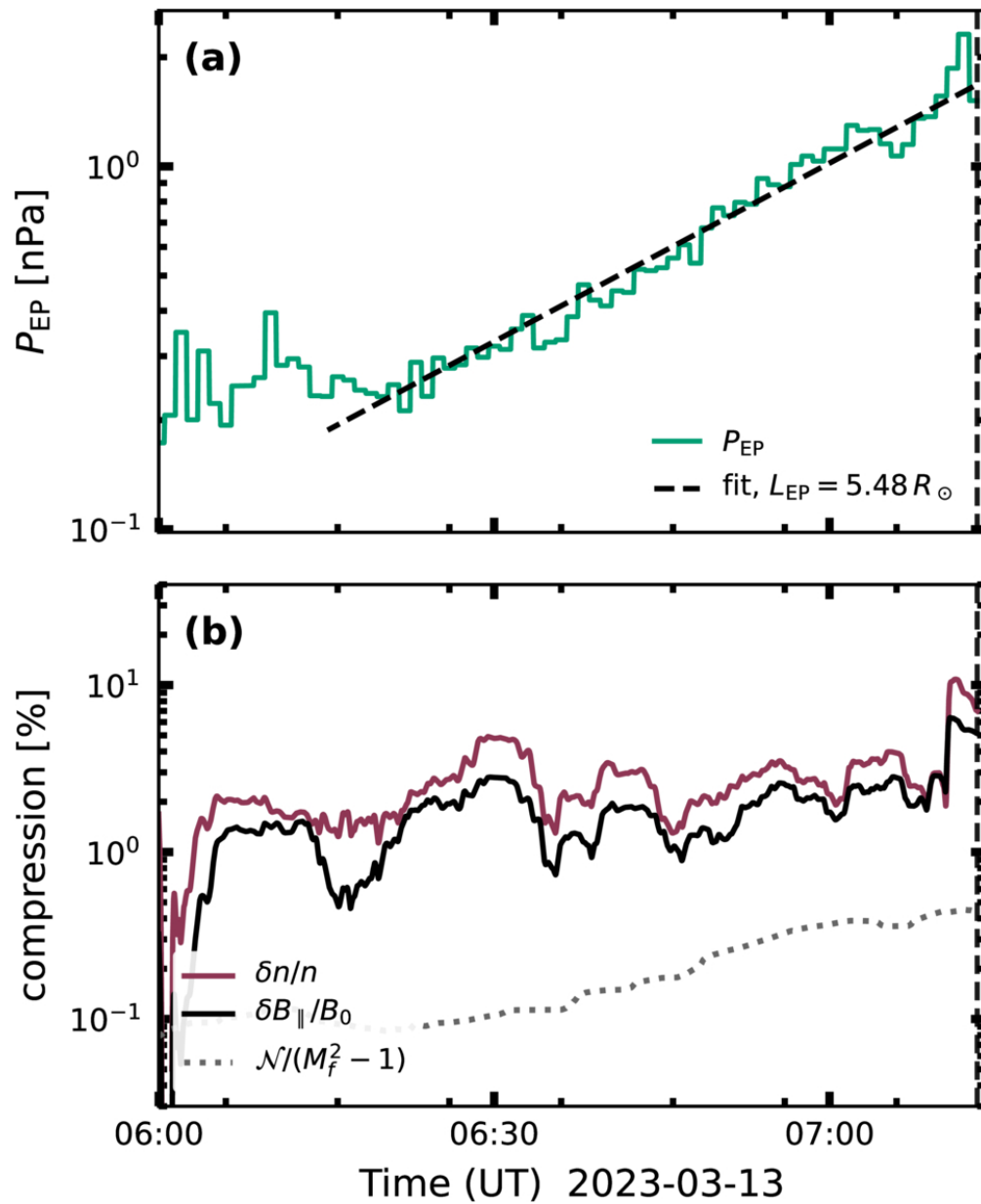
Figure 4. from I. C. Jebaraj et al 2026 Astrophys. J. Lett. 1008 doi:10.3847/2041-8213/ae9afc https://dx.doi.org/10.3847/2041-8213/ae9afc © 2026. The Author(s). Published by the American Astronomical Society.
