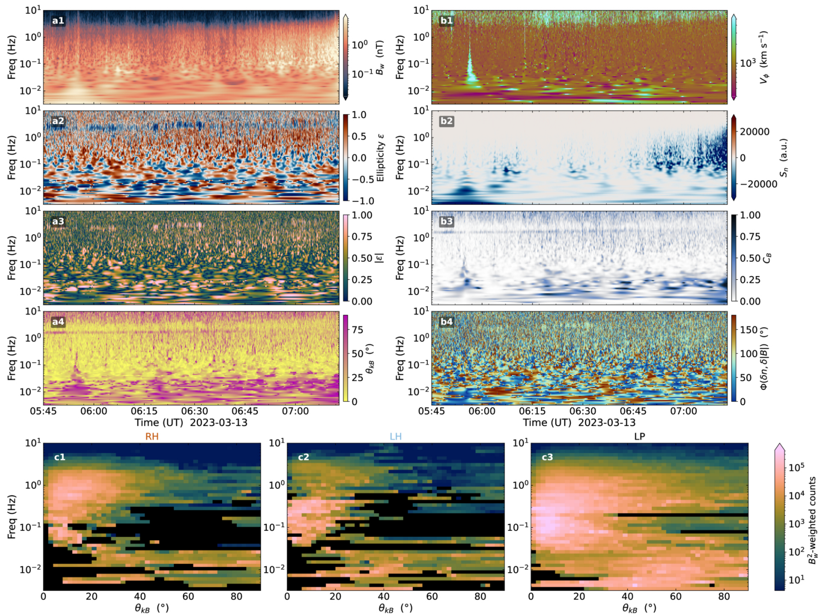
Figure 2. from I. C. Jebaraj et al 2026 Astrophys. J. Lett. 1008 doi:10.3847/2041-8213/ae9afc https://dx.doi.org/10.3847/2041-8213/ae9afc © 2026. The Author(s). Published by the American Astronomical Society.
