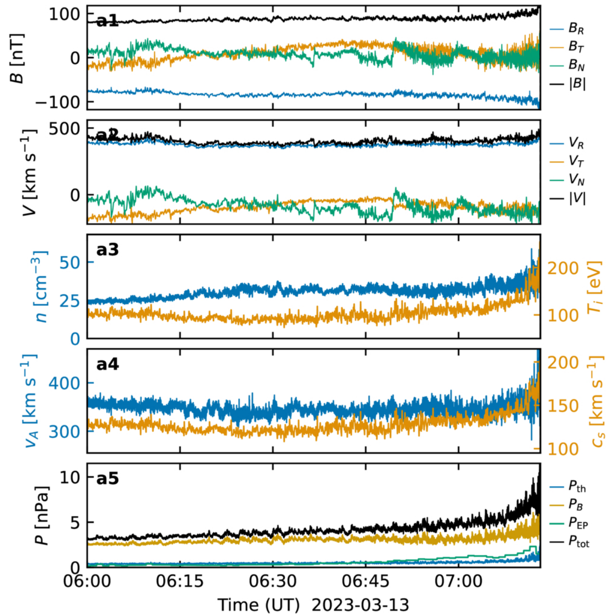
Figure 1. from I. C. Jebaraj et al 2026 Astrophys. J. Lett. 1008 doi:10.3847/2041-8213/ae9afc https://dx.doi.org/10.3847/2041-8213/ae9afc © 2026. The Author(s). Published by the American Astronomical Society.
