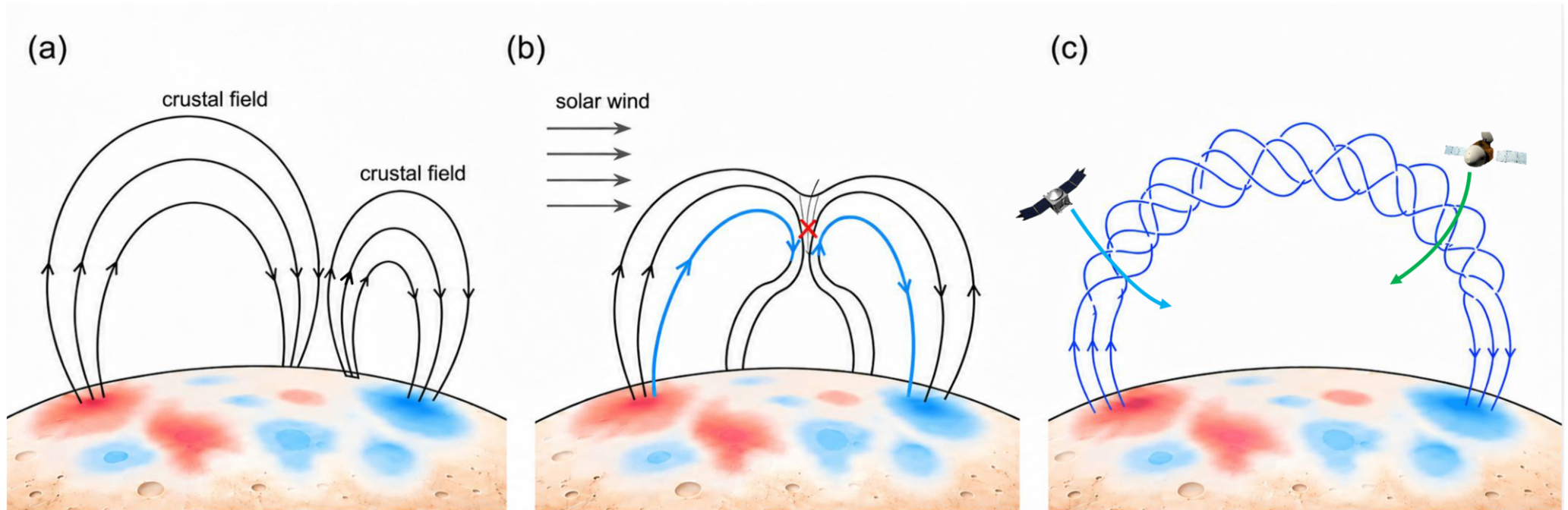
Figure 3. from Yuanzheng Wen et al 2026 Astrophys. J. Lett. 1008 doi:10.3847/2041-8213/ae9aa0 https://dx.doi.org/10.3847/2041-8213/ae9aa0 © 2026. The Author(s). Published by the American Astronomical Society.
