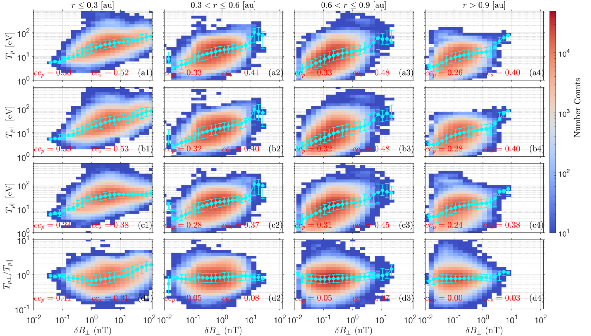
Figure 3. from Wen Liu et al 2026 Astrophys. J. Lett. 1009 doi:10.3847/2041-8213/ae9a9f https://dx.doi.org/10.3847/2041-8213/ae9a9f © 2026. The Author(s). Published by the American Astronomical Society.
