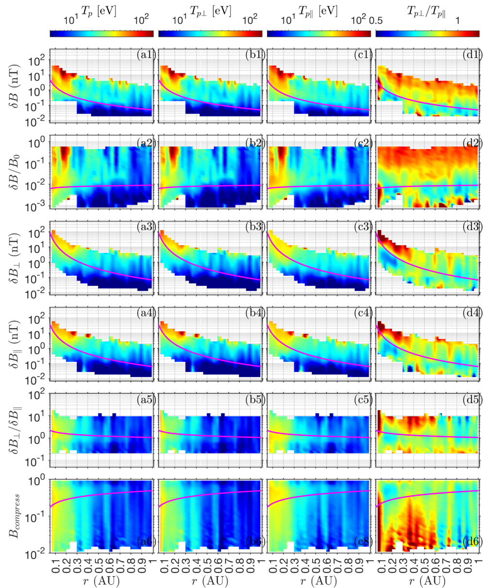
Figure 2. from Wen Liu et al 2026 Astrophys. J. Lett. 1009 doi:10.3847/2041-8213/ae9a9f https://dx.doi.org/10.3847/2041-8213/ae9a9f © 2026. The Author(s). Published by the American Astronomical Society.
