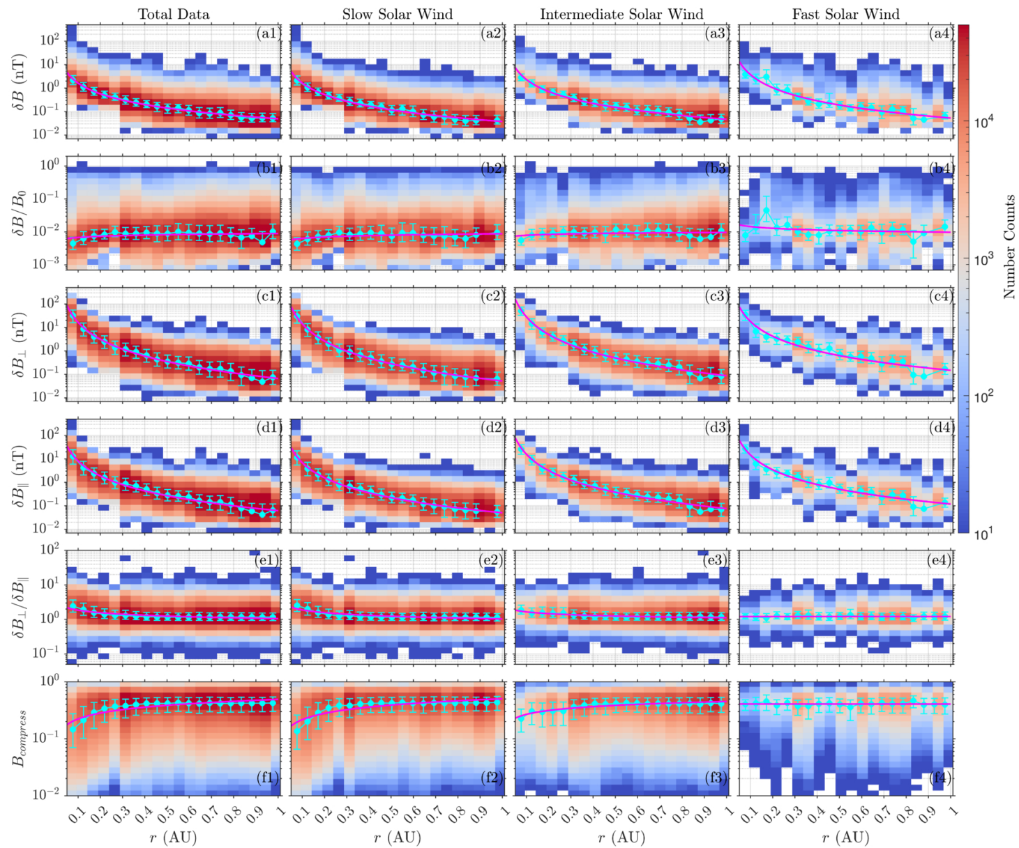
Figure 1. from Wen Liu et al 2026 Astrophys. J. Lett. 1009 doi:10.3847/2041-8213/ae9a9f https://dx.doi.org/10.3847/2041-8213/ae9a9f © 2026. The Author(s). Published by the American Astronomical Society.
