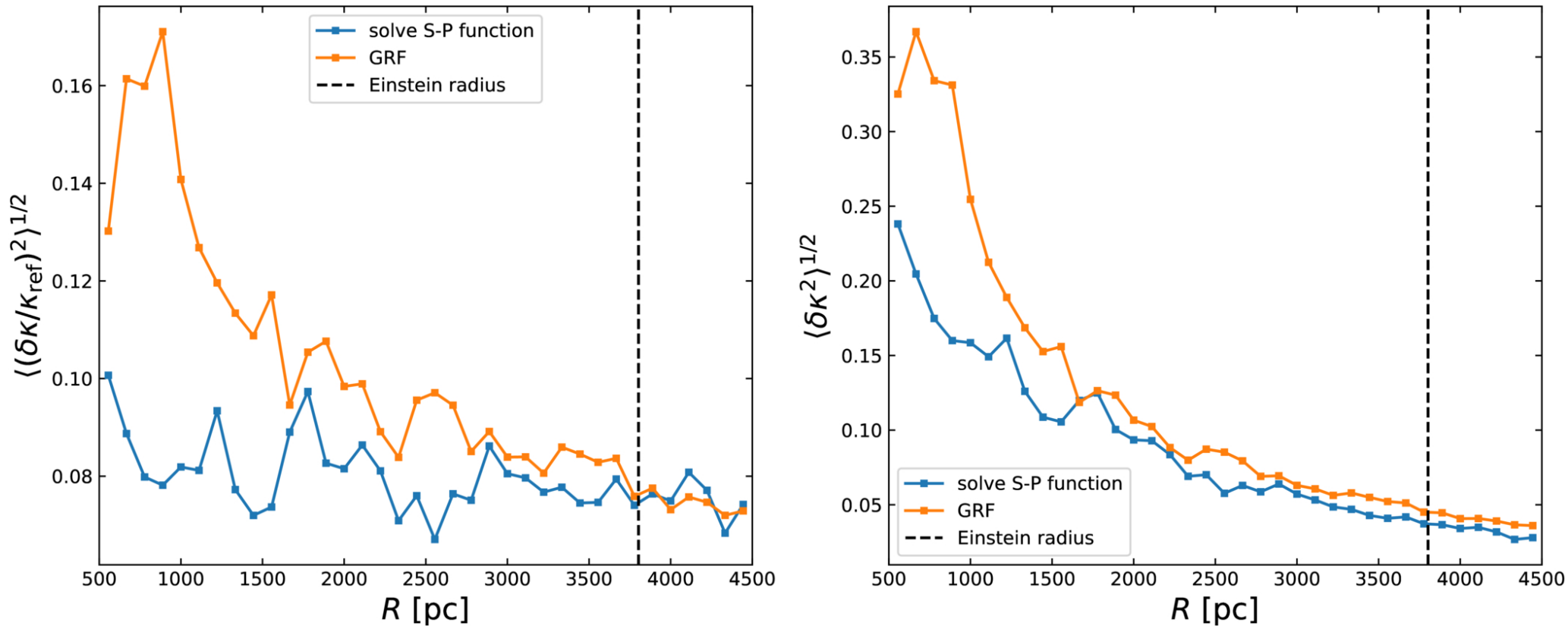
Figure A2. from Jiajun Zhou et al 2026 Astrophys. J. Lett. 1008 doi:10.3847/2041-8213/ae9a9e https://dx.doi.org/10.3847/2041-8213/ae9a9e © 2026. The Author(s). Published by the American Astronomical Society.
