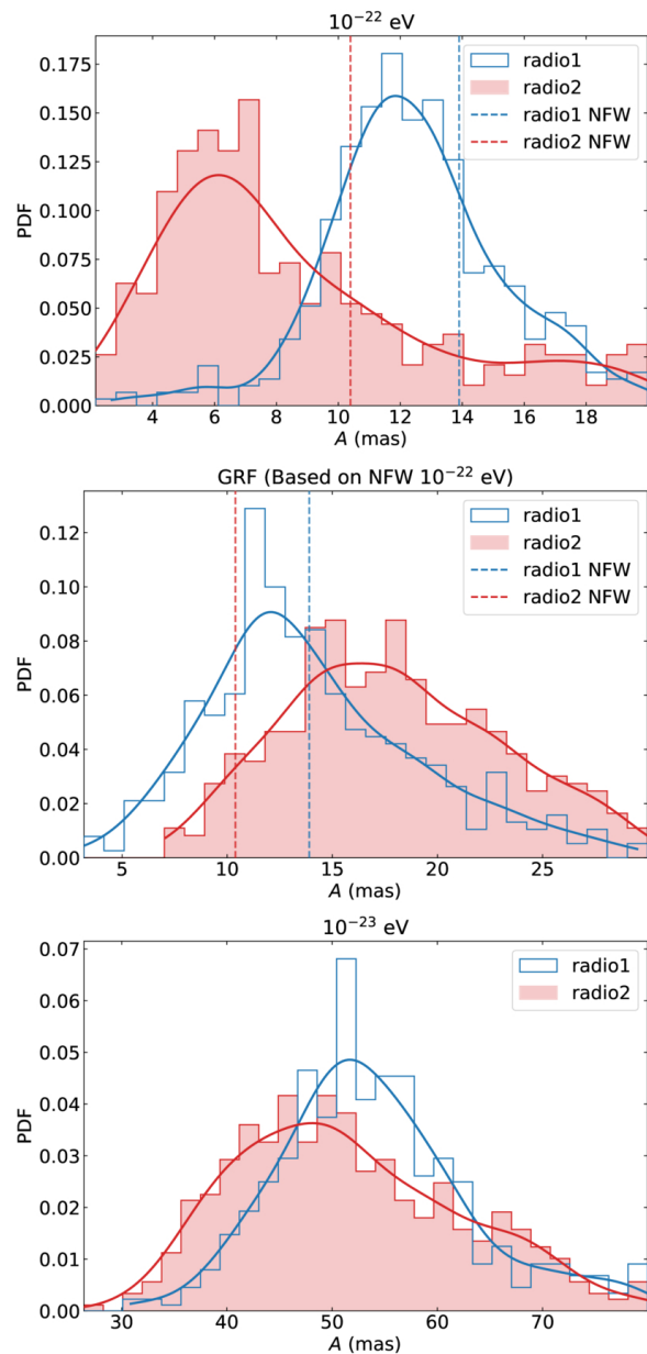
Figure 3. from Jiajun Zhou et al 2026 Astrophys. J. Lett. 1008 doi:10.3847/2041-8213/ae9a9e https://dx.doi.org/10.3847/2041-8213/ae9a9e © 2026. The Author(s). Published by the American Astronomical Society.
