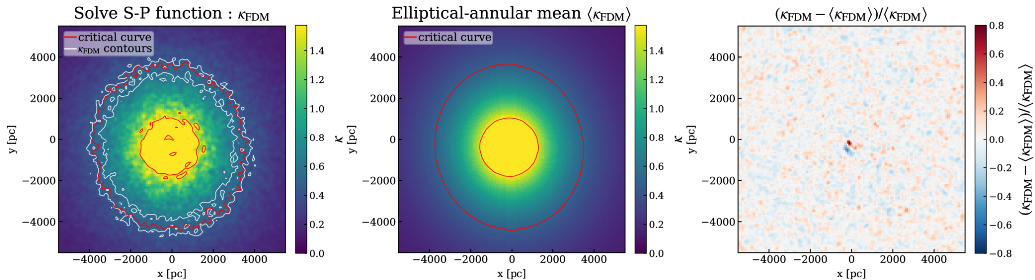
Figure 1. from Jiajun Zhou et al 2026 Astrophys. J. Lett. 1008 doi:10.3847/2041-8213/ae9a9e https://dx.doi.org/10.3847/2041-8213/ae9a9e © 2026. The Author(s). Published by the American Astronomical Society.
